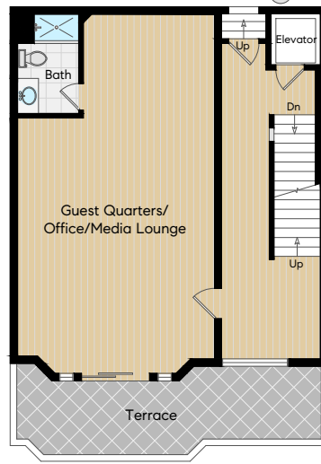
Second Level
